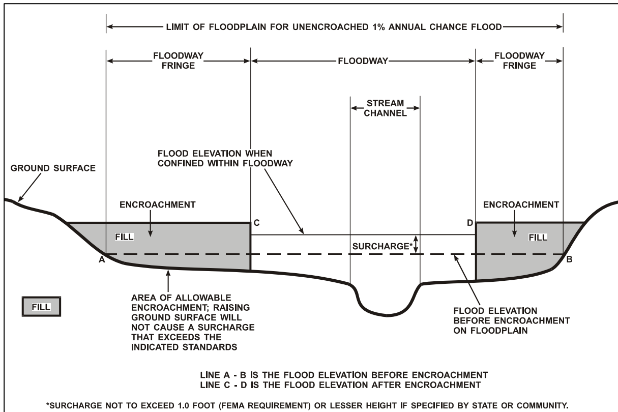
Figure 1 – Floodway Schematic
